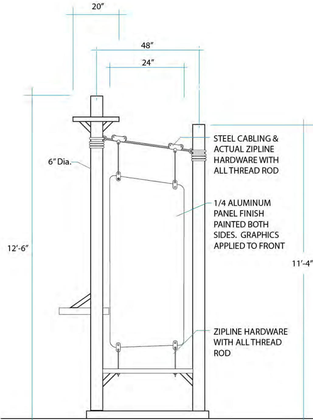
BACK VIEW
