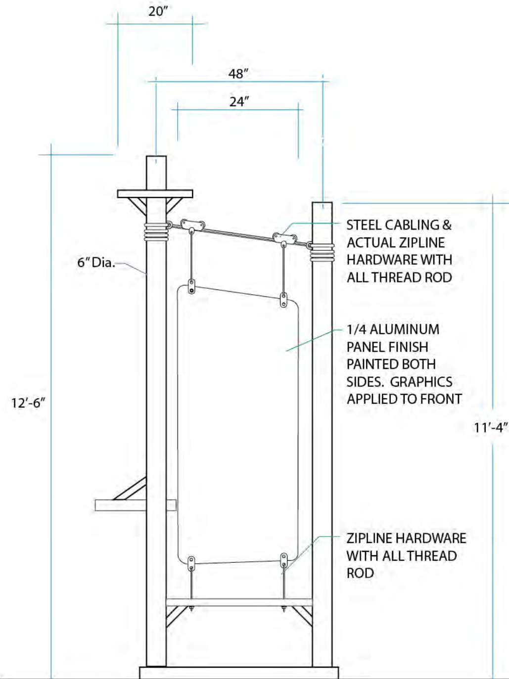
BACK VIEW
