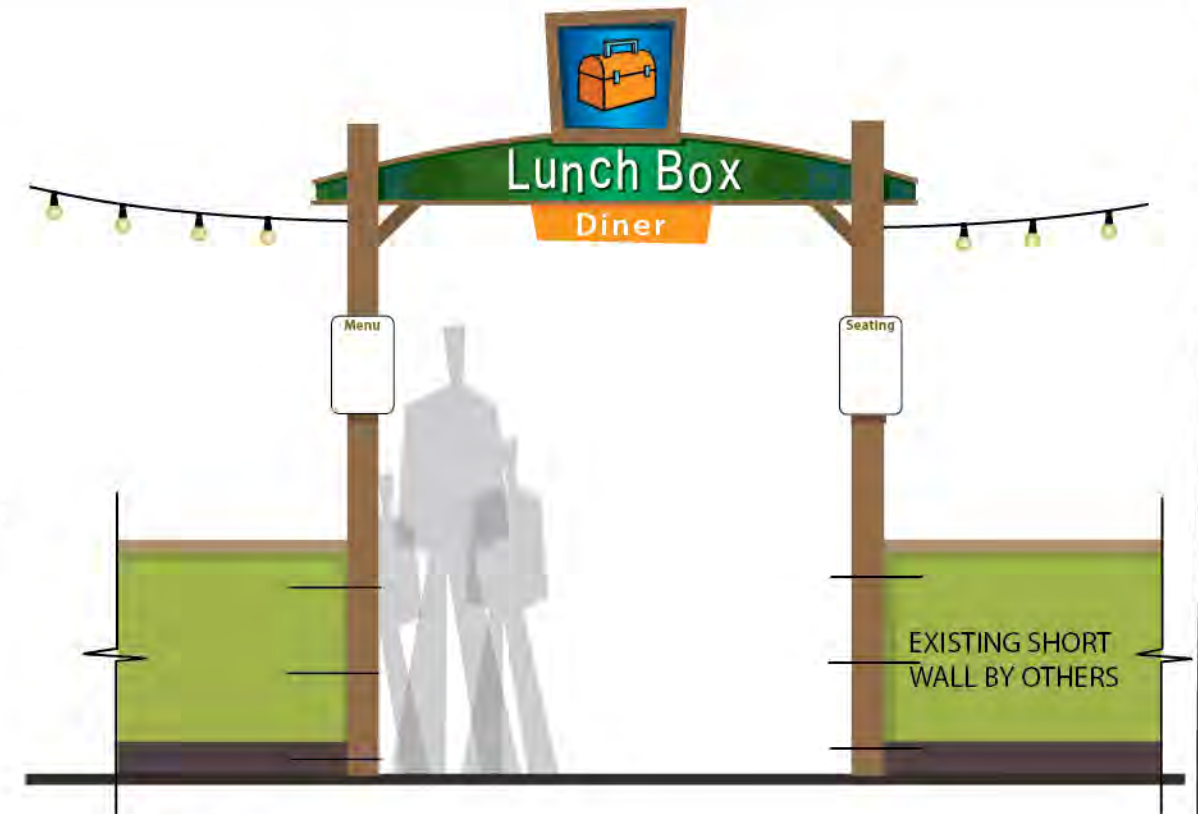
FRONT VIEW
