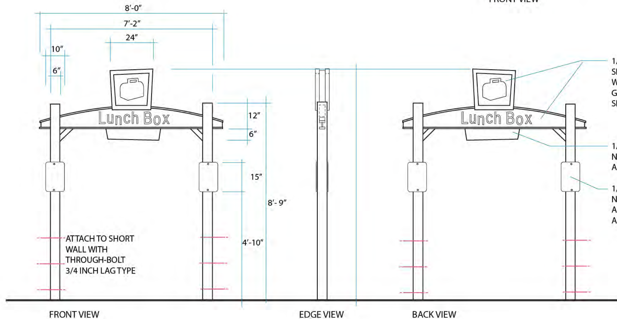
FRONT VIEW
