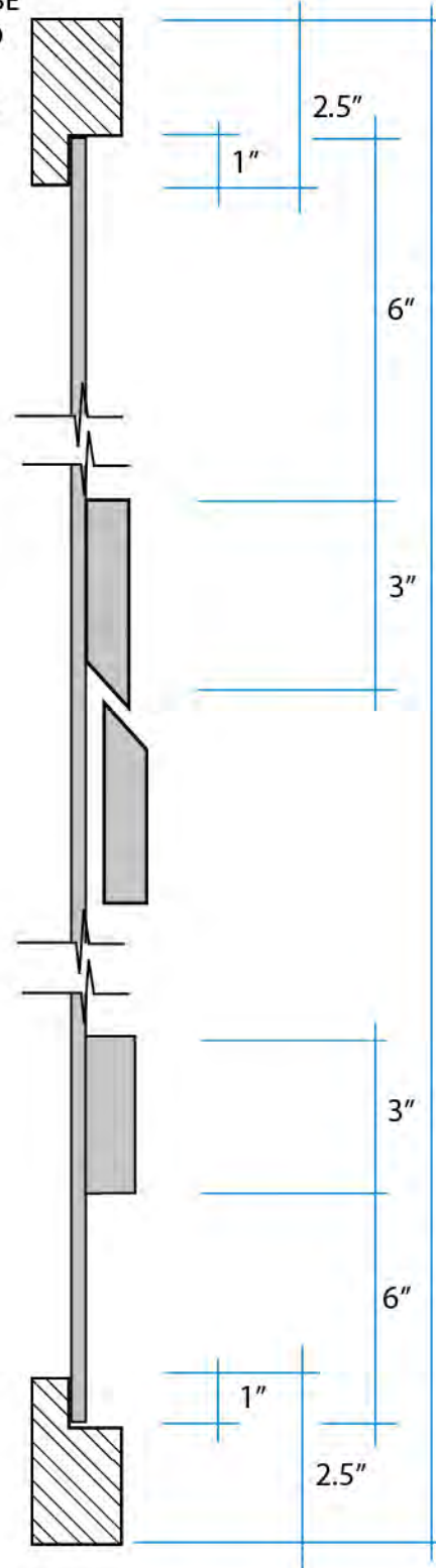
SECTION VIEW
