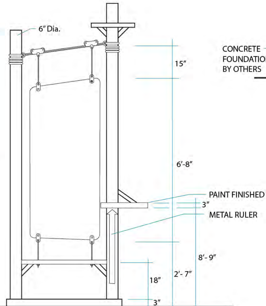
FRONT VIEW
