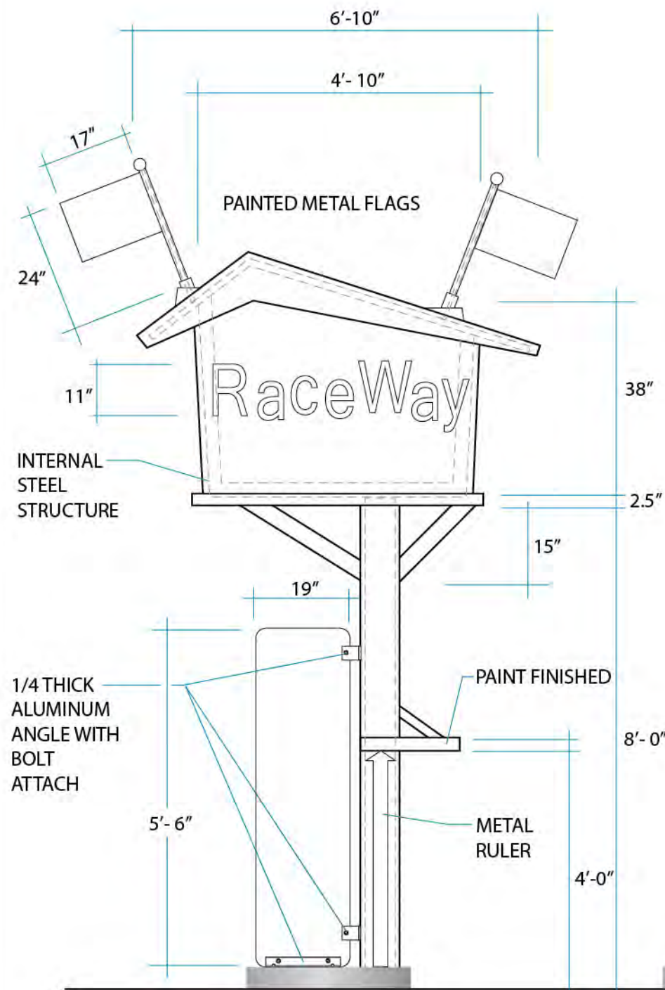
FRONT VIEW
