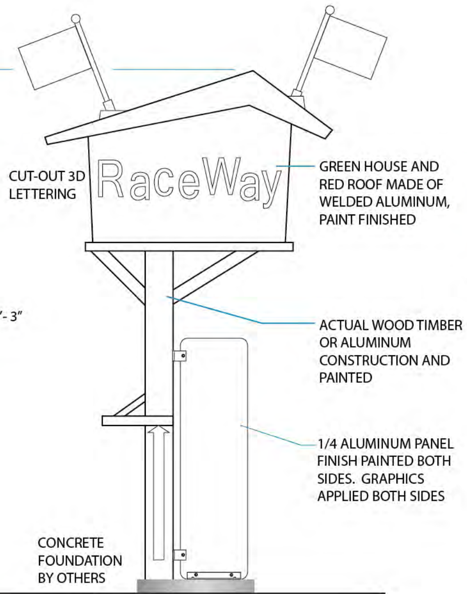
BACK VIEW
